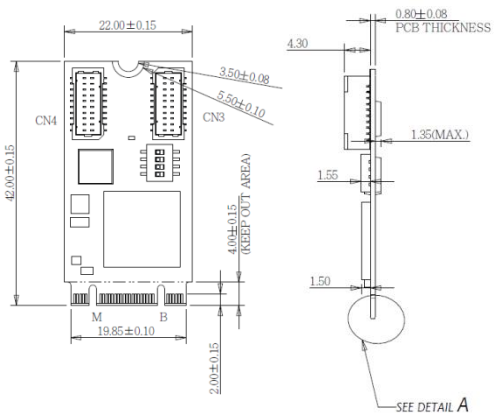
EGP2-X401-W1 (Vertical Connector)
