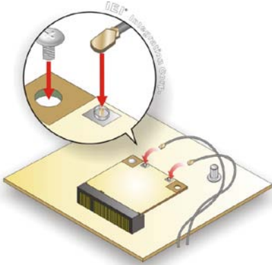
Figure 12: Removing the Retention Screw
