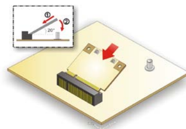
Figure 11: Inserting the WLAN Module
