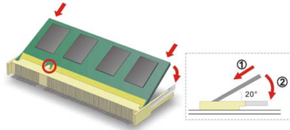
Figure 8: SO-DIMM Installation
