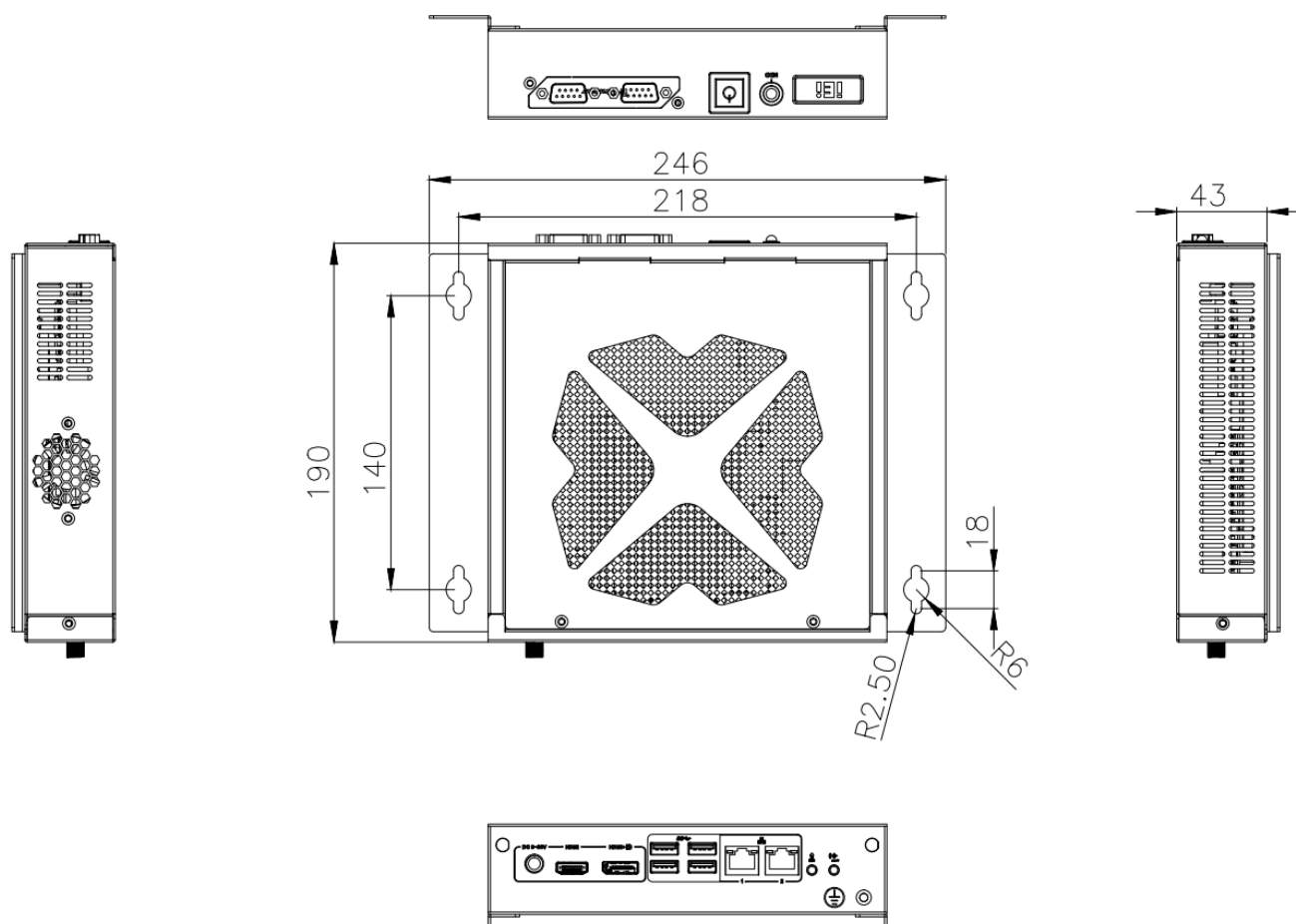
Figure 1: Dimension Drawing
