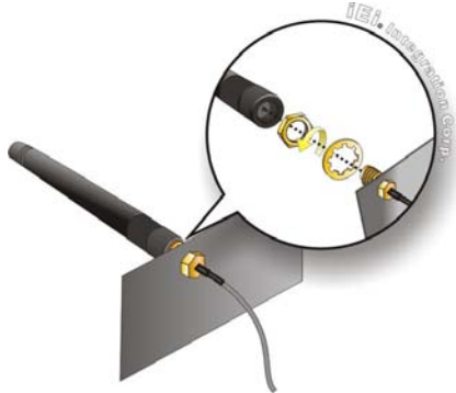
Figure 13: Securing SMA Connector and External Antenna
