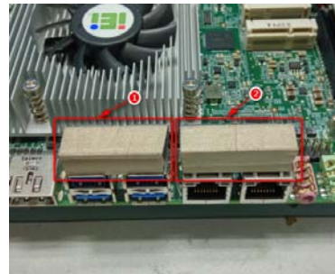
Figure 4: USB 3.0 / LAN Gaskets
