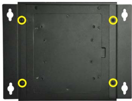
Figure 18: Wall-mount Brackets Retention Screws
