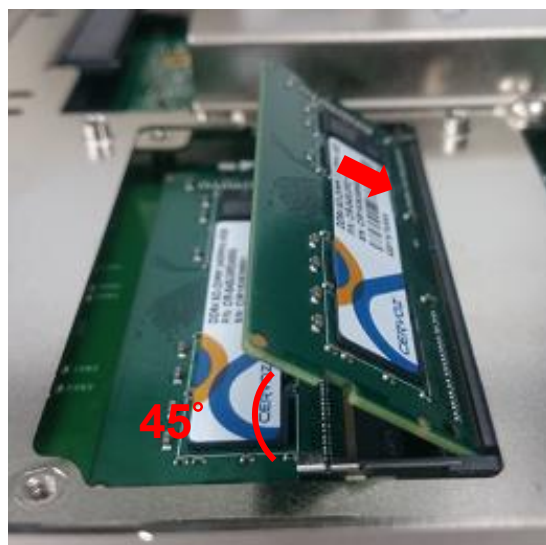
Upper socket
