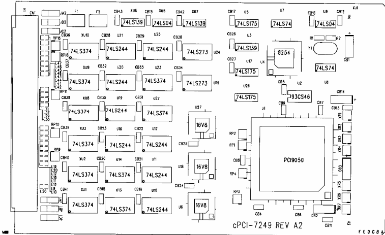
Figure 2.3.4 cPCI-7249R Layout
