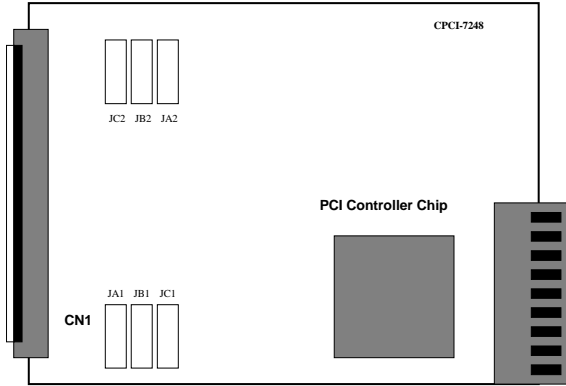
Figure 2.3.3 cPCI-7248 PCB Layout
